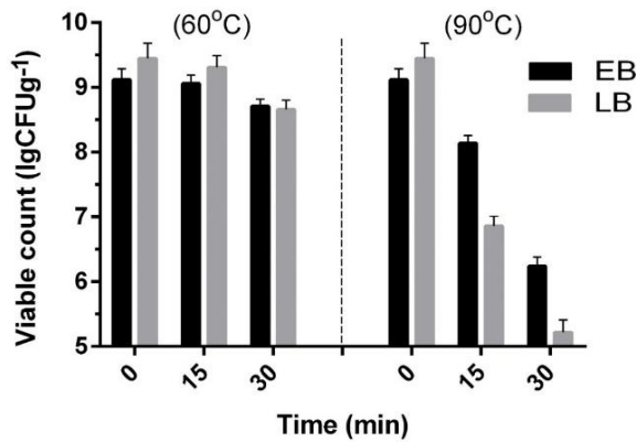
Fig. 5: Effect of heat treatment (60 and 90°C) for different intervals of time on survival of Ct . EB: Encapsulated bacteria; LB: liquid bacteria. All data were presented as mean \pm SD, n=6.
