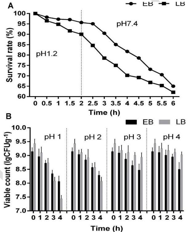
Fig. 3: In vitro characteristics of encapsulated bacteria (EB) vs. liquid bacteria (LB). A: Survival rate (%) of Ct under simulated gastric and intestinal fluid, Ct was treated with simulated gastric fluid for first 2h at pH 1.2 and then with intestinal fluid form 2-6h at pH 7.4; B: Acid tolerance, change in viable count with the passage of time at varying pH 1-4. All data were presented as mean \pm SD, n = 6.
