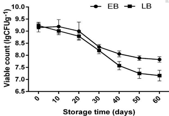
Fig. 6: Storage kinetics of Ct at 25°C for a period of 60 days. EB: Encapsulated bacteria; LB: liquid bacteria. All data were presented as mean \pm SD, n=6.
