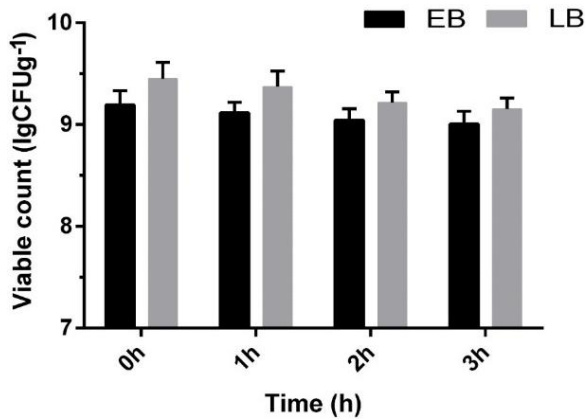
Fig. 4: Survival of Ct under bile salt (3%) treatment. EB: Encapsulated bacteria; LB: liquid bacteria. All data were presented as mean \pm SD, n=6.
