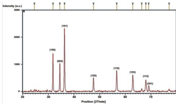
Fig. 2: X-ray diffraction Pattern of nanoscale ZnO. Different peaks showed the particle size.
