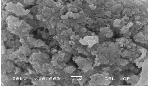
Fig. 1: Scanning electron microscopy (SEM) image of ZnO nanoparticles showed fine hexagonal wurtzite crystal structure.
