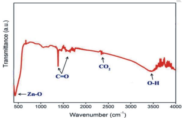
Fig. 3: FTIR spectra of associated with attached molecules with newly synthesized ZnO-NPs.
