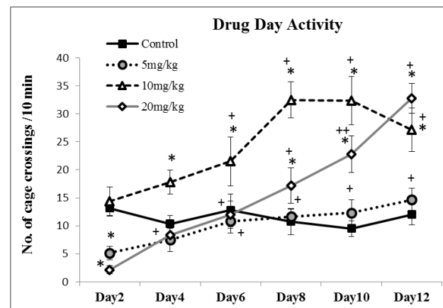
Fig. 3: Effect of all dosages of nalbuphine injection on motor behavior on drug administration day. Values represented as Means \pm S.D ( n=6 ). Significant different by Tukey's analysis: * p<0.01 from the relevant day control group, + P<0.05 , ++ P<0.01 from data of day-2 of similar administration animals following two-way ANOVA repeated measure.
