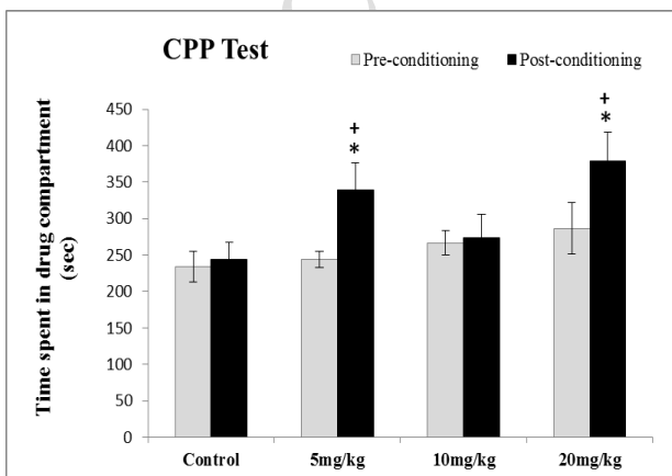
Fig. 2: Effects of different doses of nalbuphine on pre- and post-conditioning data of time spent in the drug-linked compartment. Data represented as Mean \pm SD ( n=6 ). Significant difference using Tukey's test: * P<0.01 from relative pre-conditioning data; + P<0.01 from saline injected rats using 2-way ANOVA.
