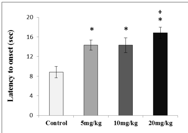
Fig. 1: Effects of different dosages of nalbuphine on heat-induced nociception. Values represented as Mean \pm SD ( n=6 ) 30 min after the first administration of nalbuphine. Significant difference by Tukey's comparison: * P<0.01 from saline injected group; + P<0.05 , ++ P<0.01 from 5 mg/kg nalbuphine injected group.
