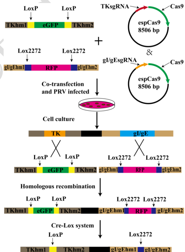
Fig. 1: Pseudorabies Gene Knockout Flow Chart. The homology arms containing TK gene, eGFP gene fragments on the LoxP site (green), homology arms containing the gE/gI gene, the RFP gene fragment at Lox2272 site (red) were constructed by the overlapping PCR method. These gene fragments and corresponding gene knock-out Cas9 recombinant plasmids were co-transfected into PK15 cells. Pseudorabies gene deletion strain was constructed by Cas9 gene editing system and homologous recombination technology, and fluorescent protein genes were introduced into the recombinant plasmid as a reporting system.
