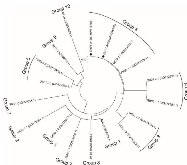
Fig. 4: Phylogenetic tree constructed from the ORF68 sequences of 2 Serbian EHV-1 isolates (marked with ◆) and the strain representatives of the 10 proposed geographic groups.
