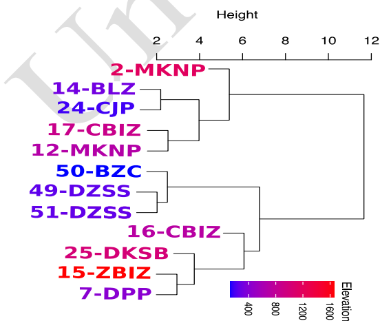
Fig. 6: Dendrogram based on morphometrical distances.
