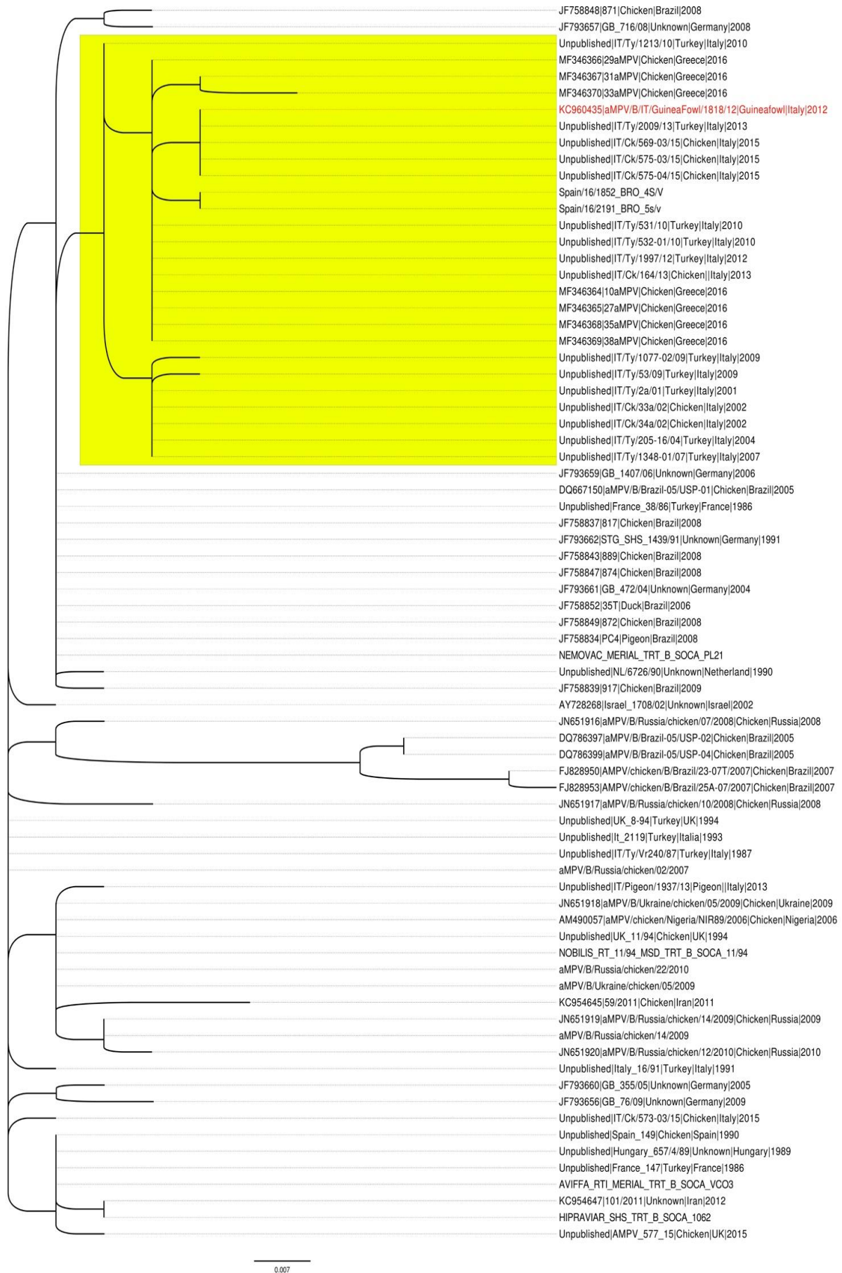
Fig. 3: Phylogenetic tree based on the alignment of partial G gene nucleotide sequences of subtype B AMPVs, constructed using the maximum likelihood method implemented in the PhyML software. A yellow box highlights a main cluster comprising Italian strains isolated after 2001, including the aMPV detected from guinea fowl (red font), Greeks and Spanish strains detected in 2016.
