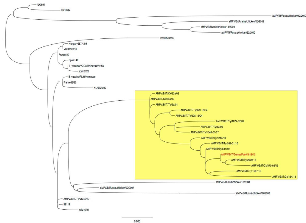
Fig. 2. Phylogenetic tree based on the alignment of complete G gene nucleotide sequences of subtype B AMPVs, constructed using the maximum likelihood method implemented in the PhyML software. A yellow box highlights a main cluster comprising all Italian strains isolated after 2001, including the aMPV detected from guinea fowl (red font).
