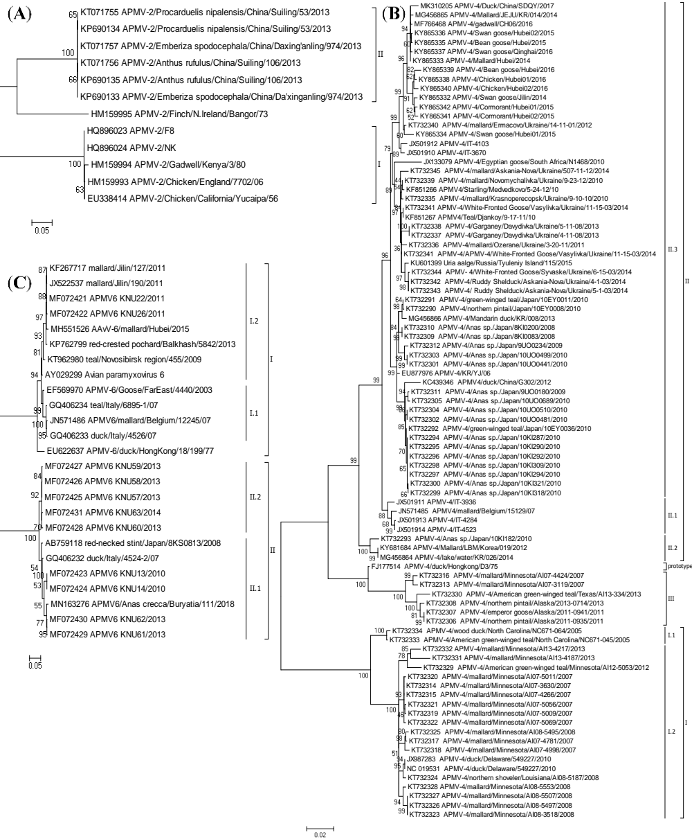
Fig. 1: Phylogenetic analysis of complete F gene sequences of so far reported strains of APMV-2 (A), APMV-4 (B), and APMV-6 (C). The Maximum Likelihood (ML) statistical method of the Tamura-Nei model with 1000 bootstraps was used for the analysis of the evolutionary relationship between strains using MEGA® 6 software.
